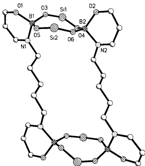
Figure 8. Molecular framework for [Salpten{B(O 2 SiPh 2 )}] 2 (6).
