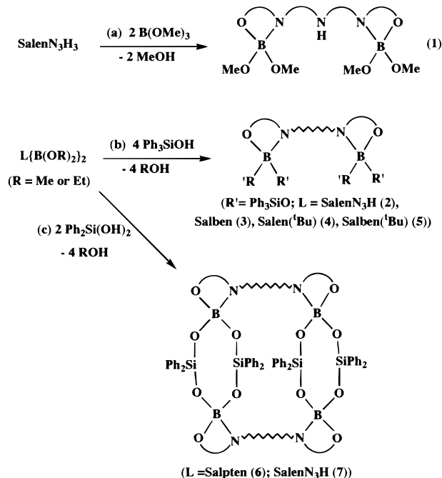
Scheme 1. General Synthesis of the Bimetallic Borate Derivatives 1–7
