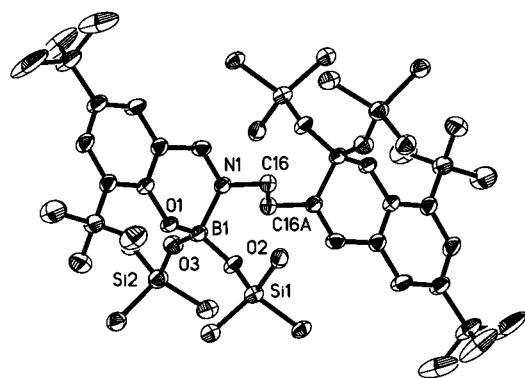
Figure 5. Molecular structure and atom numbering for Salen( t Bu)- \{B(OSiPh_3)_2\}_2 ( 4 ).
