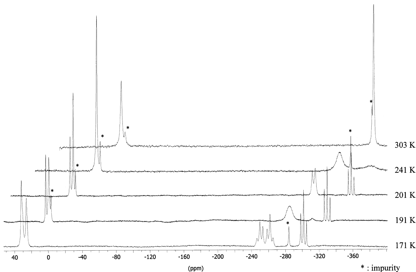
Fig. 2. 31 P{ 1 H}-NMR spectra of [(triphos)Co{(P 3 ){W(CO) 5 } 2 ] ( 4 ) at different temperatures (CD 2 Cl 2 , 81.02 MHz).
