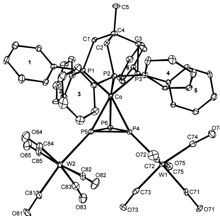
Fig. 1. A view of the [(\text{triphos})\text{Co}\{\text{P}_3\}\{\text{W}(\text{CO})_5\}_2] molecule in the structure of 4 , with 20% probability thermal ellipsoids. The phenyl rings are identified by serial numbers for clarity.
