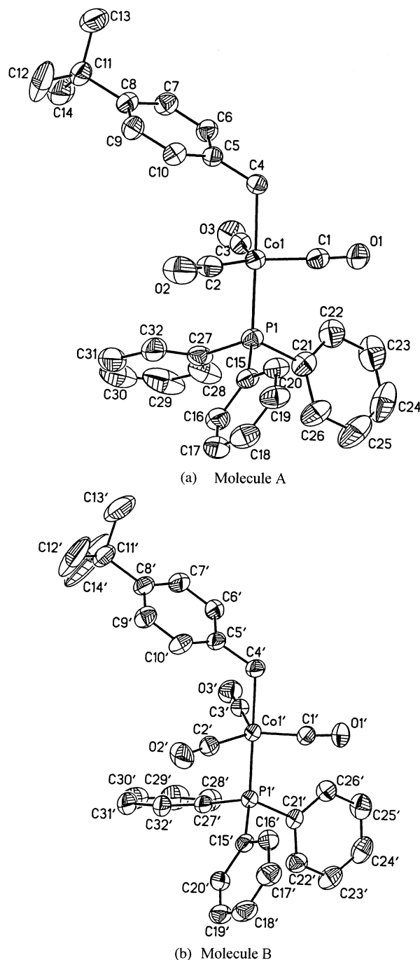
Fig. 1. ORTEP view of complex 4 with atom labels and 30% probability thermal ellipsoids. The hydrogen atoms are omitted for clarity.
