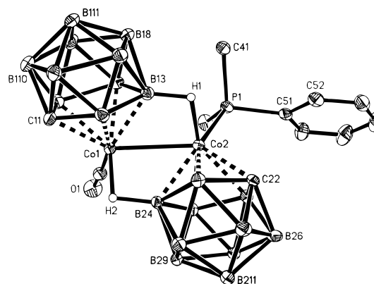
Figure 2. Molecular structure of the \alpha,\beta -isomer [Co 2 (CO)(PMe 2 Ph)( \eta^5 -7,8-C 2 B 9 H 11 ) 2 ] ( 2a ) showing the crystallographic atom-labeling scheme. Thermal ellipsoids are shown at the 40% probability level. Only the agostic hydrogen atoms are shown for clarity.
