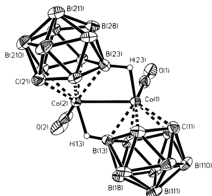
Figure 1. Molecular structure of the \alpha,\alpha -isomer [Co_2(CO)_2(\eta^5\text{-}7,8\text{-}C_2B_9H_{11})_2] ( 1a ) showing the crystallographic atom-labeling scheme. Thermal ellipsoids are shown at the 40% probability level. Only the agostic hydrogen atoms are shown for clarity.
