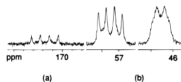
Figure 4. ^{13}\text{C}\{^1\text{H}\} NMR spectrum showing the principal peaks for the nido -carborane 6 : (a) quartet at \delta 171.7 due to the BCO carbon nucleus, (b) signals at \delta 57.5 and 46.6 due to cage CH carbon nuclei.
