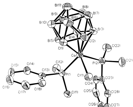
Figure 3. Molecular structure of [CoCl(PMe 2 Ph) 2 ( \eta^5 -7,8-C 2 B 9 H 11 )] ( 3 ) showing the crystallographic atom-labeling scheme. Thermal ellipsoids are shown at the 40% probability level. Hydrogen atoms are omitted for clarity.
