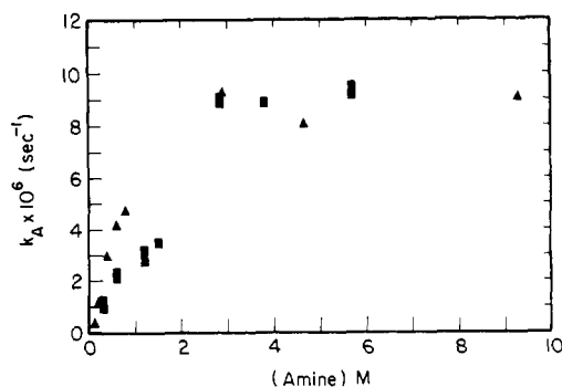
Figure 5. Rate constants ( k_A ) for formation of 1 H -azepines from irradiation of \text{PhN}_3 in hexane solutions containing DEA (triangles) or DBA (squares).
