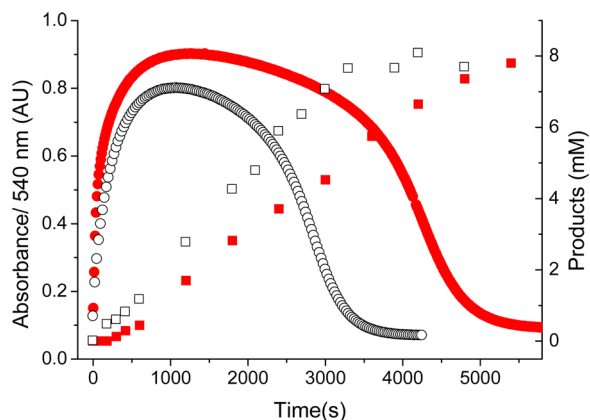
Figure 1. Time course for the oxidation of 1-octene (250 equiv) by 1.0 mM 1 and 20 equiv of \text{H}_2\text{O}_2 in \text{CH}_3\text{CN} at -40\text{ }^\circ\text{C} as monitored by the appearance and decay of 2 at 540 nm (circles) and by the formation of olefin oxidation products determined by GC (squares). The reactions were conducted in the presence of 80 (red) or 116 (black) equiv of \text{H}_2\text{O} .
