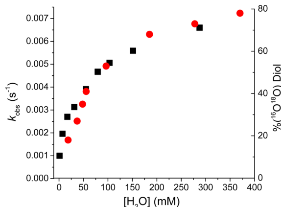
Figure 2. Water concentration dependence for the decay rate of 2 (prepared from the reaction of 1 in \text{CH}_3\text{CN} with 10 equiv of 70% \text{H}_2\text{O}_2 ) at -40\text{ }^\circ\text{C} (black squares) and the fraction of cis -diol with a single ^{18}\text{O} -label obtained in the oxidation of 1-octene by 1 and \text{H}_2\text{O}_2 in the presence of \text{H}_2^{18}\text{O} at 0\text{ }^\circ\text{C} (red circles).
