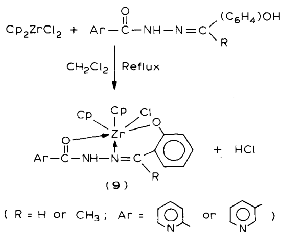
SCHEME 9. Reactions of dicyclopentadienylzirconium(IV) dichloride with salicylaldehyde or o -hydroxyacetophenone picolinoyl/nicotinoyl hydrazones in the absence of amine.
