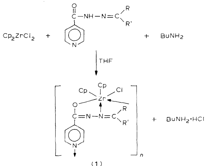
SCHEME 1. Reactions of dicyclopentadienylzirconium(IV) dichloride with acetone or acetophenone isonicotinoyl hydrazones.
