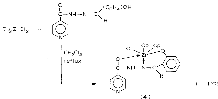
SCHEME 4. Reactions of dicyclopentadienylzirconium(IV) dichloride with salicylaldehyde or o -hydroxy-acetophenone isonicotinoyl hydrazones in the absence of amine.
