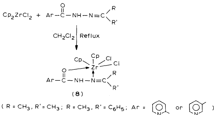
SCHEME 8. Reactions of dicyclopentadienylzirconium(IV) dichloride with acetone or acetophenone picolinoyl/nicotinoyl hydrazones in the absence of amine.
