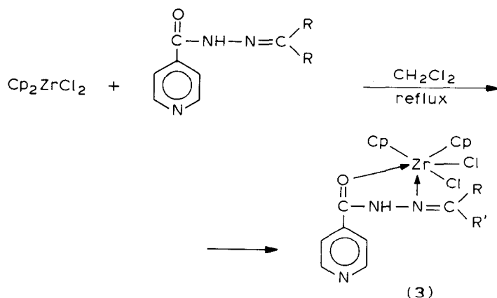
SCHEME 3. Reactions of dicyclopentadienylzirconium(IV) dichloride with acetone or acetophenone isonicotinoyl hydrazones in the absence of amine.
