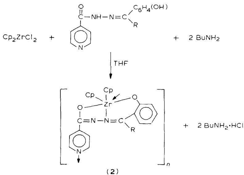
SCHEME 1. Reactions of dicyclopentadienylzirconium(IV) dichloride with acetone or acetophenone isonicotinoyl hydrazones.
