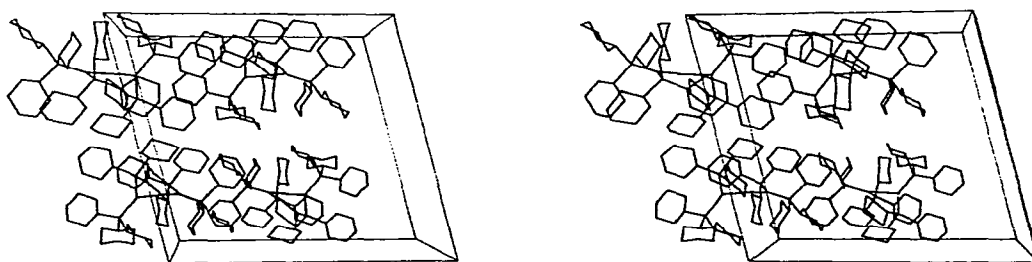
Fig. 5. Stereoscopic view of a unit cell content, viewed along b ; the a axis is horizontal.
