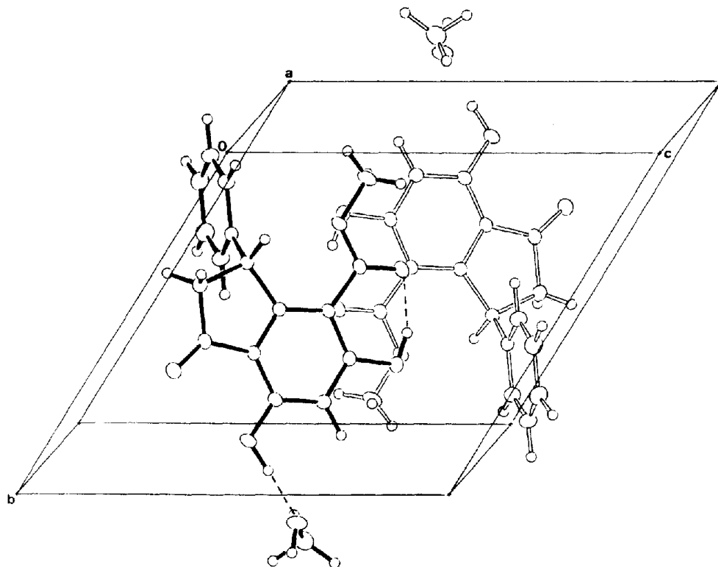
Fig. 2. Crystal packing in the unit cell of 7.
