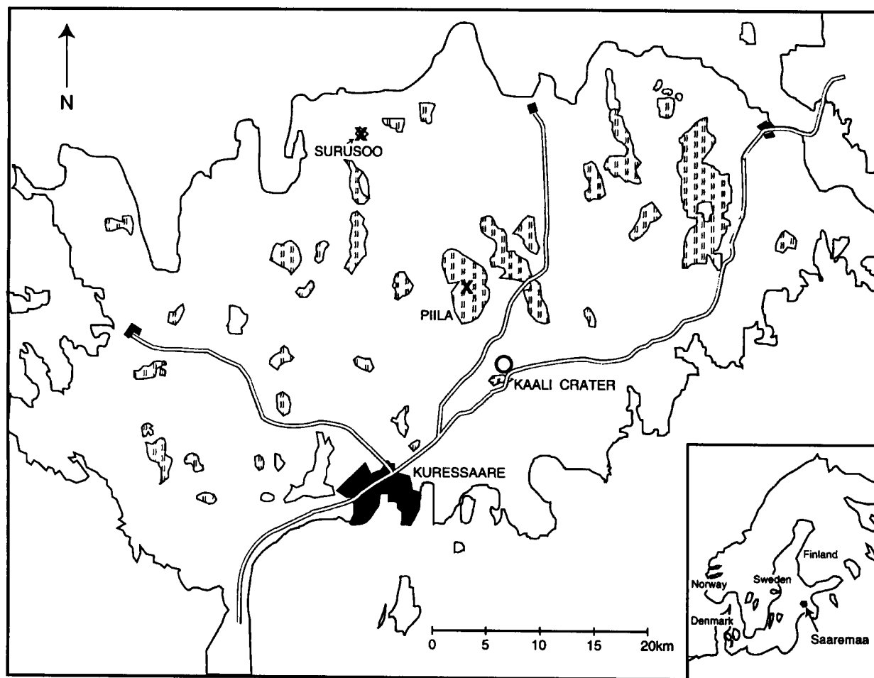
FIG. 1. Map showing the position of the Kaalijärv meteorite craters and positions of the peat sampling sites, the Piila and Surusoo mires on the Island of Saaremaa (Ösel), Estonia.
