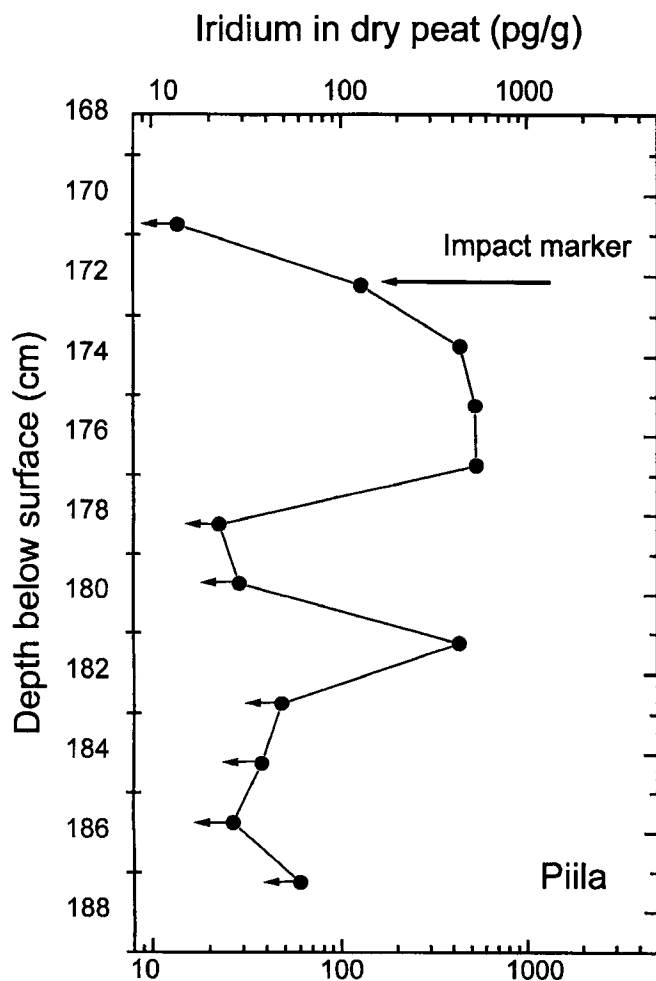
FIG. 2. Iridium concentration as a function of depth determined in the ash fraction of the peat core from Piila. Arrows indicate upper limits. The top of the Ir-enriched layer marks the impact.
