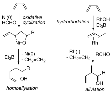
Scheme 4. Reductive Coupling Reaction of Aldehyde with Diene Promoted by \text{Ni}/\text{Et}_3\text{B} versus \text{Rh}/\text{Et}_3\text{B}
