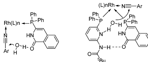
Figure 6. Hypothetical structures, directing the nucleophilic attack of water.
