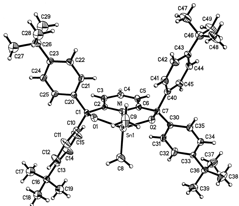
Fig. 2. Molecular structure for compound 2c .
