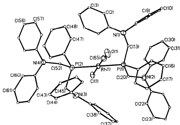
Fig. 2. A perspective view of \text{Rh}(\text{Ph}_2\text{NCH}_2\text{P}(\text{Ph})\text{CH}_2\text{NPh}_2)_2(\text{CO})\text{Cl} (6).
