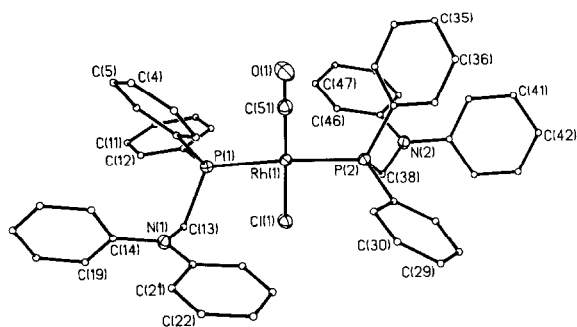
Fig. 1. A perspective view of \text{Rh}(\text{Ph}_2\text{PCH}_2\text{NPh}_2)_2(\text{CO})\text{Cl} (5).
