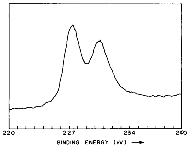
Fig. 2. XPS spectrum in the Mo 3d region.
