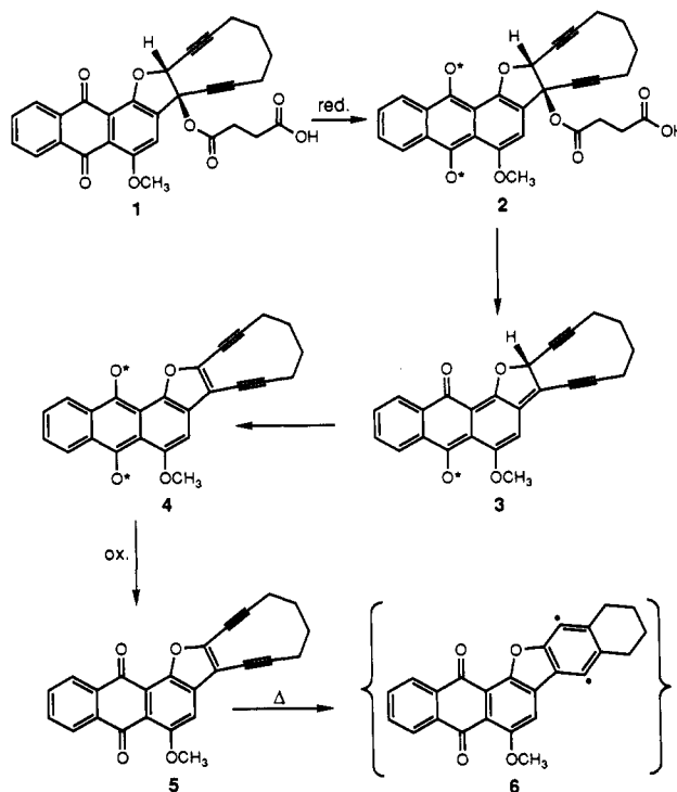
Scheme I. Proposed Transformation of Anthraquinone 1 to (Z)-Enediyne 5 and Cyclization of the Latter to Biradical 6 a
