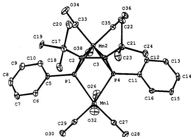
Figure 2. ORTEP drawing of one molecule of 4a . Selected bond lengths (Å) are as follows: Mn(1)–P(1) = 2.325(2), Mn(1)–P(4) = 2.326(2), Mn(2)–P(1) = 2.297(2), Mn(2)–P(4) = 2.295(2), Mn(2)–C(2) = 2.185(7), Mn(2)–C(3) = 2.208(7), P(1)–C(2) = 1.828(7), C(2)–C(3) = 1.438(9), C(3)–P(4) = 1.830(7). Bond angles (deg): P(1)–Mn(1)–P(4) = 66.73(7), Mn(1)–P(1)–C(2) = 111.4(2), P(1)–C(2)–C(3) = 108.1(5), C(2)–C(3)–P(4) = 107.5(4), Mn(1)–P(4)–C(3) = 111.1(2), Mn(1)–P(1)–Mn(2) = 109.92(8), Mn(1)–P(4)–Mn(2) = 109.97(8), Mn(2)–P(1)–C(2) = 62.7(2), Mn(2)–C(2)–C(3) = 71.8(4), Mn(2)–C(3)–P(4) = 68.5(2).
