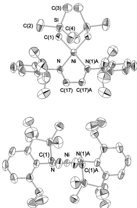
Fig. 1. ORTEP diagrams for the molecular structure of {DAD(H,H)}Ni(CH 2 SiMe 3 ) 2 ( 3 ). Thermal ellipsoids are drawn at the 50% probability level. Hydrogen atoms have been omitted for the sake of clarity.
