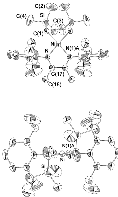
Fig. 2. ORTEP diagrams for the molecular structure of {DAD(Me,Me)}Ni(CH 2 SiMe 3 ) 2 ( 4 ). Thermal ellipsoids are drawn at the 50% probability level. Hydrogen atoms have been omitted for the sake of clarity.
