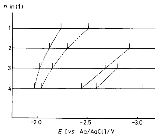
Figure 2. Correlation diagram for the redox states in (1a)–(d).
