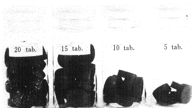
Fig. 7. Effect of Number of Tablets on Whisker Growth
