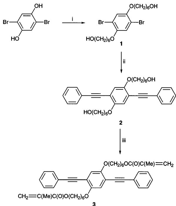
Scheme 1 Reagents and conditions: i, \text{HO}(\text{CH}_2)_6\text{Br} (2 equiv.), butanone, \text{K}_2\text{CO}_3 , heat; ii, \text{PhC}\equiv\text{CH} (2 equiv.), piperidine, \text{Pd}(\text{PPh}_3)_4 , \text{CuI} , 90^\circ\text{C} , 36 h; iii, \text{CH}_2=\text{C}(\text{Me})\text{COCl} (2 equiv.), \text{CH}_2\text{Cl}_2 , \text{Et}_3\text{N}
