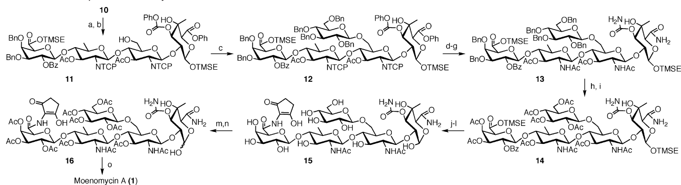
Scheme 2. Completion of the Synthesis a
