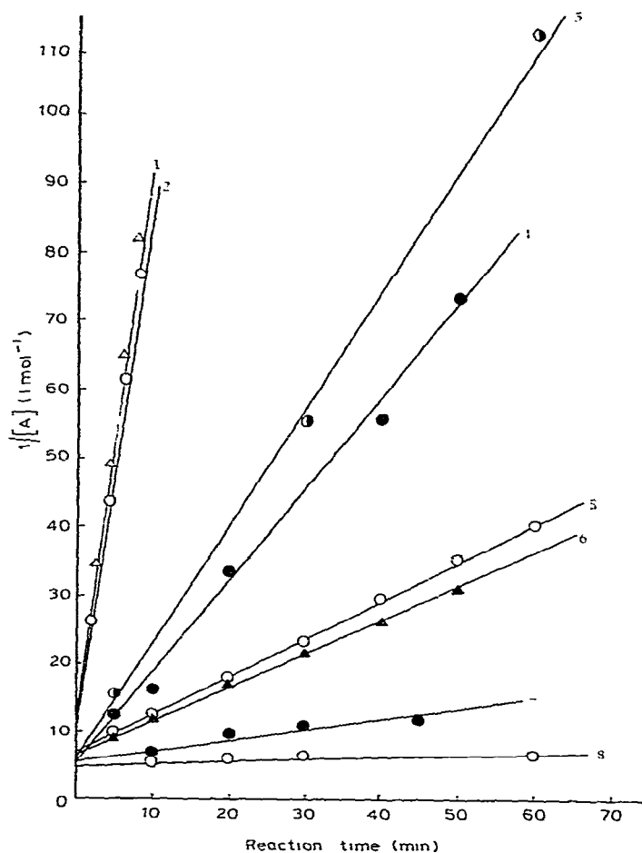
Fig. 1. Second order plots: ( k_2 values in \text{l mol}^{-1} \text{s}^{-1} \times 10^2 ): (1) \text{Ph}_3\text{C}\cdot\text{BF}_4 in \text{CH}_2\text{Cl}_2 at 0^\circ\text{C} (7.14); (2) \text{Ph}_3\text{COH} in \text{CH}_2\text{Cl}_2 at 0^\circ\text{C} (catalytic quantity of \text{HBF}_4\cdot\text{Et}_2\text{O} ) (6.81); (3) \text{Ph}_3\text{COH} in \text{CH}_2\text{Cl}_2/\text{MEK} (1/1) at 0^\circ\text{C} (1.45); (4) \text{Ph}_3\text{COH} in \text{CH}_2\text{Cl}_2/\text{MEK} (2/1) at 0^\circ\text{C} (1.10); (5) \text{Ph}_3\text{COH} in \text{CH}_2\text{Cl}_2/\text{MEK} (4/1) at 0^\circ\text{C} (0.475); (6) \text{Ph}_3\text{COH} in \text{CH}_2\text{Cl}_2/\text{acetone} (4/1) at 0^\circ\text{C} (0.425); (7) \text{Ph}_3\text{COH} in \text{CH}_2\text{Cl}_2/\text{acetylacetone} (4/1) at 0^\circ\text{C} (0.135); (8) \text{Ph}_3\text{COH} in \text{CH}_2\text{Cl}_2 at 20^\circ\text{C} (0.025).
