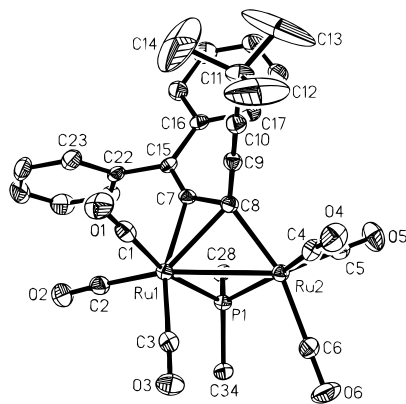
Figure 1. Molecular structure of [\text{Ru}_2(\text{CO})_6(\mu\text{-}\eta^1, \eta^2_{\alpha, \beta}\text{-C}(\text{C}\equiv\text{CBu})\equiv\text{C}=\text{CPh}_2)(\mu\text{-PPh}_2)] ( 2a ) with the non-hydrogen atom labeling scheme. For clarity, only the ipso carbons of the P -phenyl rings are drawn. Important bond lengths (Å) and angles (deg) not mentioned in the text are as follows: \text{Ru}(1)\text{--Ru}(2) = 2.825(1) , \text{Ru}(1)\text{--C}(7) = 2.170(3) , \text{Ru}(1)\text{--C}(8) = 2.297(3) , \text{C}(8)\text{--C}(9) = 1.438(5) , \text{C}(10)\text{--C}(11) = 1.475(5) ; \text{C}(8)\text{--C}(7)\text{--C}(15) = 144.6(3) , \text{C}(7)\text{--C}(8)\text{--C}(9) = 114.3(3) , \text{C}(8)\text{--C}(9)\text{--C}(10) = 178.9(4) , \text{Ru}(1)\text{--P}(1)\text{--Ru}(2) = 73.6(1)^\circ .
