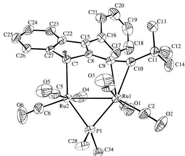
Figure 2. Molecular structure of [\text{Ru}_2(\text{CO})_6\{\mu\text{-}\eta^1, \eta^2\text{-CH}(\text{C}_6\text{H}_4)\text{C}(\text{Ph})=\text{CC}\equiv\text{CBu}^t\}(\mu\text{-PPh}_2)] ( 3 ) with the non-hydrogen atom labeling scheme. For clarity, only the ipso carbons of the P -phenyl rings are drawn. Important bond lengths (Å) and angles (deg) not mentioned in the text are as follows: \text{Ru}(1)\text{--Ru}(2) = 2.8928(4) , \text{C}(7)\text{--C}(8) = 1.478(4) , \text{C}(8)\text{--C}(9) = 1.428(4) , \text{C}(10)\text{--C}(11) = 1.496(5) , \text{C}(8)\text{--C}(15) = 1.387(4) , \text{C}(15)\text{--C}(22) = 1.455(5) , \text{C}(22)\text{--C}(27) = 1.399(5) , \text{C}(27)\text{--C}(7) = 1.475(4) , \text{C}(7)\text{--C}(8)\text{--C}(9) = 122.5(3) , \text{C}(8)\text{--C}(9)\text{--C}(10) = 166.5(3) , \text{C}(9)\text{--C}(10)\text{--C}(11) = 151.6(3) , \text{Ru}(1)\text{--P}(1)\text{--Ru}(2) = 76.88(3) , \text{C}(8)\text{--C}(15)\text{--C}(22) = 106.9(3) , \text{C}(15)\text{--C}(22)\text{--C}(27) = 109.2(3) , \text{C}(22)\text{--C}(27)\text{--C}(7) = 109.2(3)^\circ .
