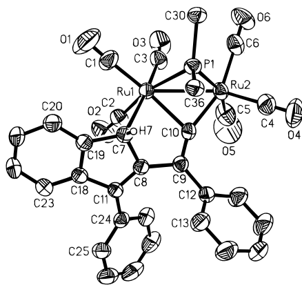
Figure 3. Molecular structure of [\text{Ru}_2(\text{CO})_6\{\mu\text{-}\eta^1, \eta^2\text{-C}=\text{C}(\text{Ph})\text{C}=\text{C}(\text{Ph})(\text{C}_6\text{H}_4)\text{CH}\}(\mu\text{-PPh}_2)] ( 4 ) with the non-hydrogen atom labeling scheme. For clarity, only the ipso carbons of the P -phenyl rings are drawn. Important bond lengths (Å) and angles (deg) not mentioned in the text are as follows: \text{Ru}(1)\text{--Ru}(2) = 2.826(1) , \text{Ru}(1)\text{--C}(7) = 2.291(3) , \text{C}(7)\text{--C}(8) = 1.482(5) , \text{C}(8)\text{--C}(9) = 1.481(5) , \text{C}(8)\text{--C}(11) = 1.362(4) , \text{C}(11)\text{--C}(18) = 1.464(5) , \text{C}(18)\text{--C}(19) = 1.415(4) , \text{C}(19)\text{--C}(7) = 1.482(5) , \text{Ru}(1)\text{--C}(7)\text{--C}(8) = 99.9(2) , \text{C}(7)\text{--C}(8)\text{--C}(9) = 114.6(2) , \text{C}(8)\text{--C}(9)\text{--C}(10) = 110.7(3) , \text{C}(9)\text{--C}(10)\text{--Ru}(1) = 118.3(3) , \text{Ru}(1)\text{--C}(10)\text{--Ru}(2) = 84.7(1) , \text{Ru}(1)\text{--P}(1)\text{--Ru}(2) = 73.4(1)^\circ .
