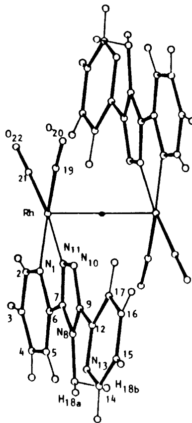
Fig. 1. View of the dimeric units centrosymmetrically related ( i = x̄, ȳ, z̄ ) showing the atomic numbering of complex IX . Carbon symbols are omitted for clarity.
