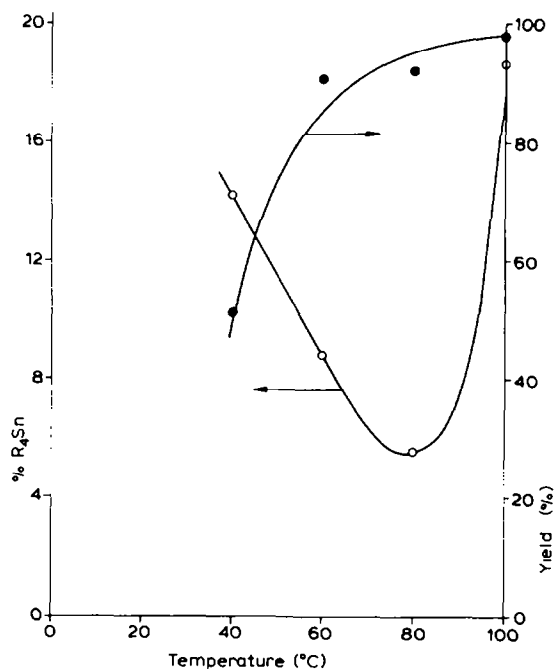
Fig. 1. The effect of temperature upon yield (●), R_3SnCl + R_4Sn ; and upon product composition (○), % R_4Sn ; in the reaction between (\beta\text{-CBE})_2SnCl_2 (0.022 mol) and Zn (0.031 mol) in toluene (20 ml) ( R = \beta\text{-CBE} ). Reaction times; 336 h at 40°C, 2 h at 60°C, 1 h at 80°C, and 0.5 h at 100°C.
