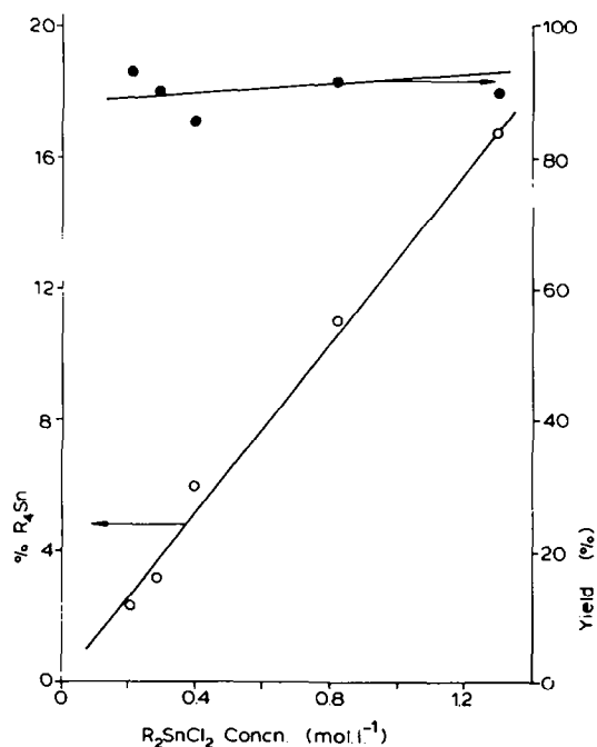
Fig. 2. The effect of concentration upon yield (●), R_3SnCl + R_4Sn ; and upon product composition (○), % R_4Sn ; in the reaction between (\beta\text{-CBE})_2SnCl_2 (0.022 mol) and Zn (0.031 mol) in toluene at 80°C ( R = \beta\text{-CBE} ).
