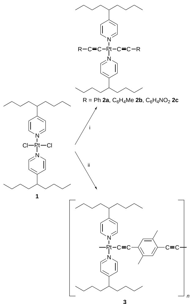
Scheme 1 i, 3 equiv. HC≡CR (R = Ph 2a , C 6 H 4 Me 2b , C 6 H 4 NO 2 2c ), catalytic amount of CuI in Pr i 2 NH, CH 2 Cl 2 , stirred at room temp. for 1 h; ii, 1 equiv. HC≡CC 6 H 2 (Me) 2 C≡CH, catalytic amount of CuI in Pr i 2 NH, CH 2 Cl 2 , stirred at room temp. for 1 h
