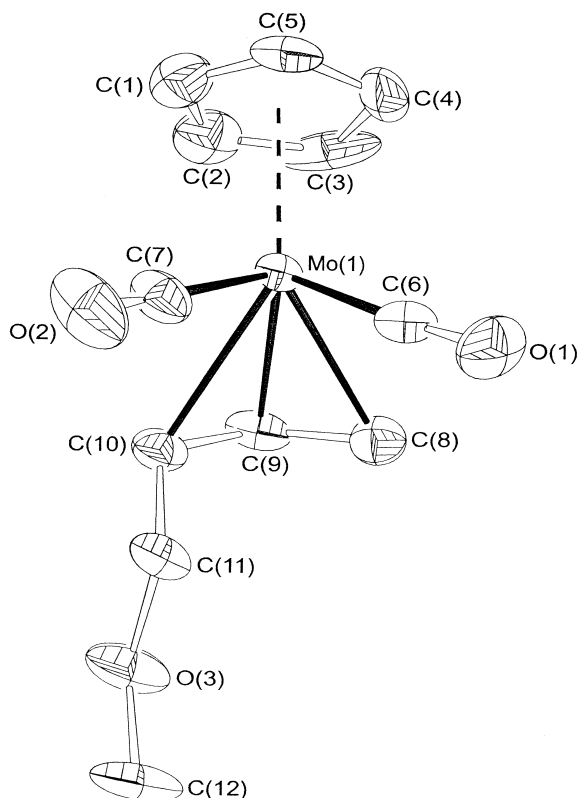
Fig. 3. The molecular structure of 7 showing the numbering scheme used in the text and tables.
