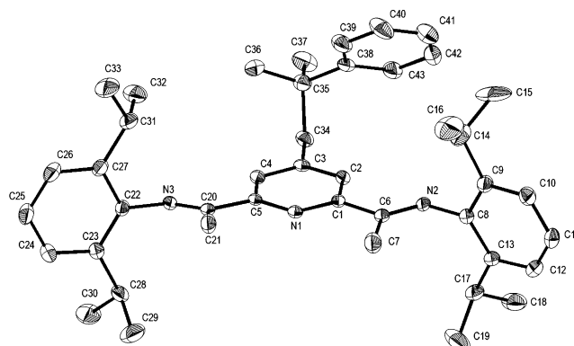
Figure 1. ORTEP drawing of compound 2a .
