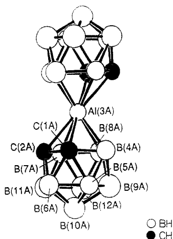
Figure 5. Structure of [commo-3,3'-Al(3,1,2-AlC_2B_9H_{11})_2]^- ( [5]^- ) with hydrogen atoms omitted for clarity.
