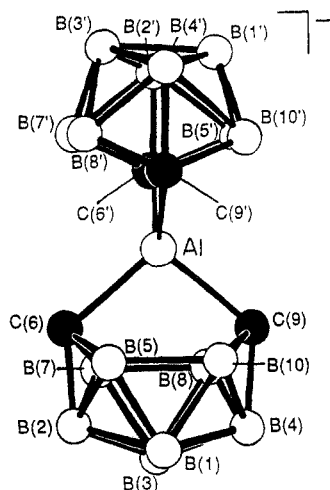
Figure 11. Structure of [\text{Al}(\text{nido-6,9-C}_2\text{B}_8\text{H}_{10})_2]^- ( [10]^- ) with hydrogen atoms omitted.
