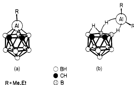
Figure 1. Structures of 3-R-3,1,2-AlC 2 B 9 H 11 (R = Et, 1a ; R = Me, 1b ) and nido -9,10-(μ-H) 2 -9,10-AlR 2 -7,8-C 2 B 9 H 11 (R = Et, 2 ; R = Me, 2' ) shown schematically.
