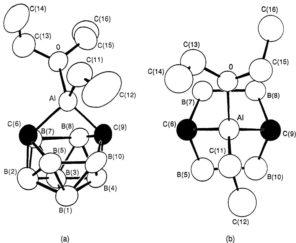
Figure 9. (a) Structure of nido -6,9-(μ-AlEt(OEt 2 ))-6,9-C 2 B 8 H 10 (8) with hydrogen atoms omitted. (b) View of 8 along the C(6)–Al–C(9) plane with atoms B(1), B(2), B(3), and B(4) and all hydrogen atoms omitted.
