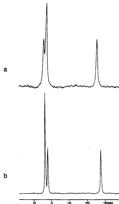
Figure 10. 11 B{ 1 H} NMR spectra (160.5 MHz) of (a) nido -6,9-(μ-AlEt(OEt 2 ))-6,9-C 2 B 8 H 10 (8) and (b) [Al( nido -6,9-C 2 B 8 H 10 ) 2 ] - ([10] - ) in toluene- d 8 solution.
