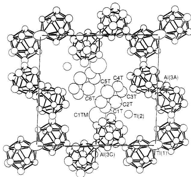
Figure 6. Unit cell diagram for Tl[5] \cdot 2/3 C_7H_8 . The Al(3B) atoms are hidden behind Tl(1) in this view.
