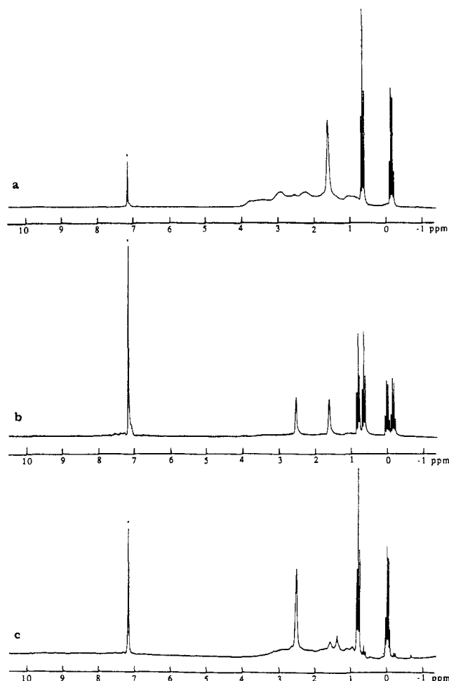
Figure 3. 1 H NMR spectra (25 °C, 200.1 MHz) of 3-Et-3,1,2-AlCl 2 B 9 H 11 ( 1a ) in benzene- d 6 solution (a) before heating and (b) after 12 h at 85 °C and (c) of 4 in benzene- d 6 solution.
