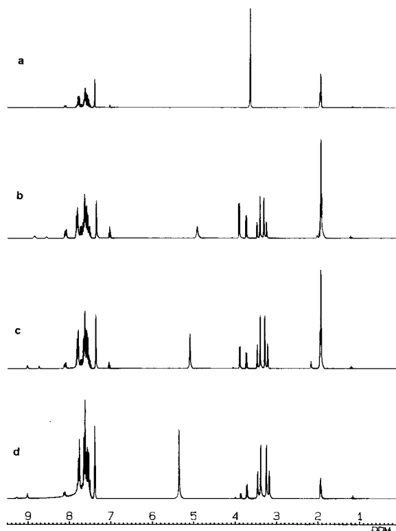
Figure. a) 270 MHz pmr spectrum of 4 in acetonitrile- d 3 after deuterium oxide exchange; b) 270 MHz pmr spectrum of 4 in acetonitrile- d 3 at 65°; c) same as in b except at 25°; d) same as in b except at -35°.
