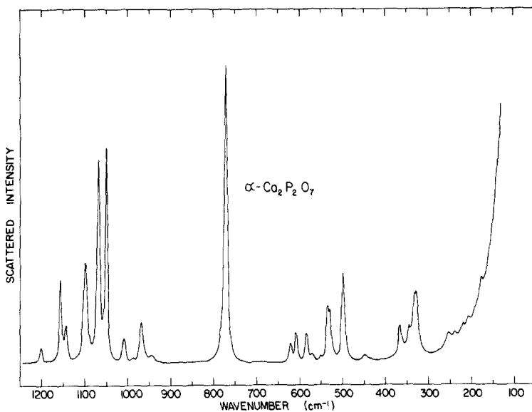
FIG. 2. The Raman spectrum of \alpha - \text{Ca}_2\text{P}_2\text{O}_7 .
