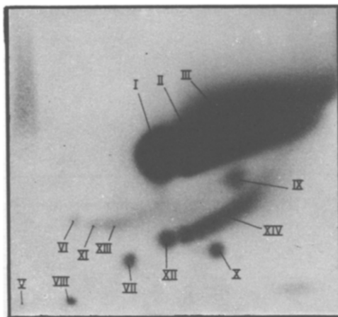
FIG. 1 Two-dimensional TLC of primary oxidation products from 2,6-dimethylphenol
