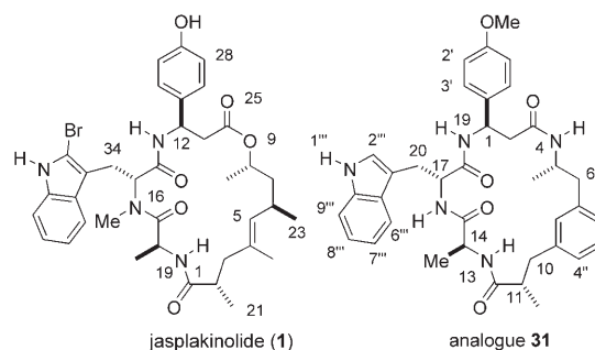
Figure 5. Structures for the natural compound jasplakinolide and the 19-membered ring analogue 31 with the numbering systems used.
