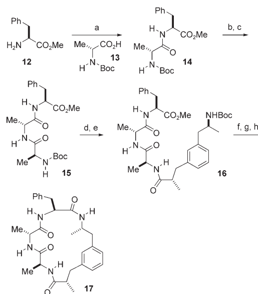
Scheme 2. Preparation of the geodiamolide analogue 17 . a) DCC, HOBT, amino acid 13 , THF, 0 \rightarrow 23^{\circ}\text{C} , 12 h (80 %); b) TFA, \text{CH}_2\text{Cl}_2 , 23^{\circ}\text{C} ; c) EDCI, HOBT, Boc-L-Ala-OH, \text{Et}_3\text{N} , THF/ \text{CH}_2\text{Cl}_2 5:1, 0 \rightarrow 23^{\circ}\text{C} , 16 h (75 %); d) TFA, \text{CH}_2\text{Cl}_2 , 23^{\circ}\text{C} ; e) TBTU, HOBT, amino acid 4 , i\text{Pr}_2\text{NEt} , DMF, 23^{\circ}\text{C} , 3 h (95 %, crude); f) NaOH, THF/ \text{H}_2\text{O} , 23^{\circ}\text{C} , 3 h; g) TFA, \text{CH}_2\text{Cl}_2 , 23^{\circ}\text{C} , 1 h; h) TBTU, HOBT, i\text{Pr}_2\text{NEt} , DMF, 23^{\circ}\text{C} , 14 h (50 %, three steps).
