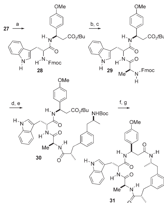
Scheme 5. Synthesis of the tripeptide 29 , coupling with amino acid 4 , and formation of macrocycle 31 . a) Fmoc-D-Trp-OH, DCC, HOBT, THF, -10 \rightarrow 0^{\circ}\text{C} , 12 h (91%); b) \text{Et}_2\text{NH} , THF, 0 \rightarrow 23 ^{\circ}\text{C} , 80 min (78%); c) Fmoc-L-Ala-OH, DCC, HOBT, THF, 0 ^{\circ}\text{C} , 12 h (97%); d) \text{Et}_2\text{NH} , THF, 0 \rightarrow 23 ^{\circ}\text{C} , 80 min (85%); e) DCC, HOBT, THF, amino acid 4 , -20 \rightarrow 23^{\circ}\text{C} , 8.5 h (92%); f) TFA, \text{CH}_2\text{Cl}_2 , 0 \rightarrow 23 ^{\circ}\text{C} , 1.5 h; g) TBTU, HOBT, i\text{Pr}_2\text{NEt} , DMF, 23 ^{\circ}\text{C} , 14 h (92%, two steps).
