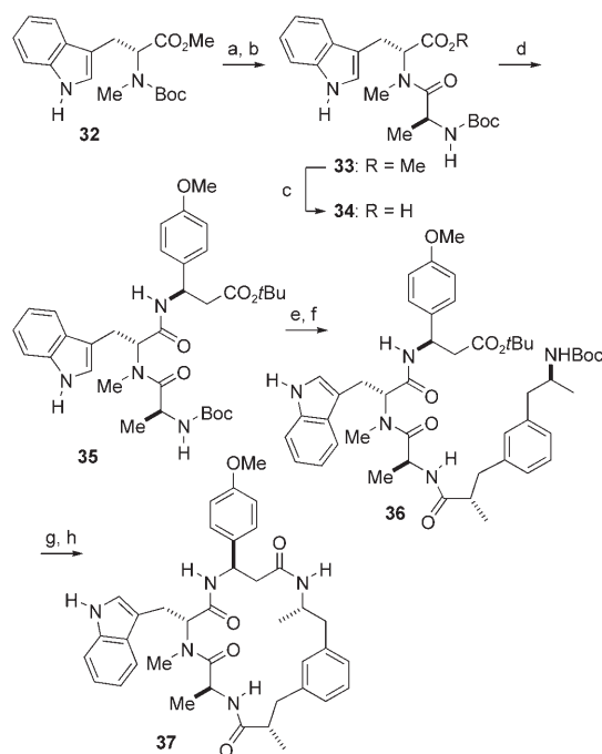
Scheme 6. Synthesis of the macrocycle 37 with a N-methyl group at the tryptophan amino acid. a) TFA, CH 2 Cl 2 , 23 °C, 1 h (68 %); b) Boc-L-Ala-OH, DCC, HOBT, THF, 0 → 23 °C, 14 h (59 %); c) NaOH, THF, 23 °C, 2 h (74 %); d) amino acid 27 , DCC, HOBT, −20 → 0 °C, 12 h (96 %); e) TBDMSOTf, 2,6-lutidine, CH 2 Cl 2 , 0 °C, 1 h, then add H 2 O (56 %); f) amino acid 4 , DCC, HOBT, THF, −20 → 23 °C, 18.5 h (60 %); g) TFA, CH 2 Cl 2 , 0 → 23 °C, 1.5 h; h) TBTU, HOBT, i Pr 2 NEt, 23 °C, 14 h (45 %, two steps).
