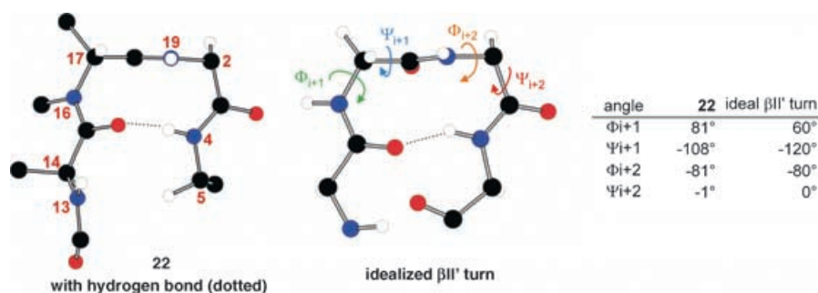
Figure 8. Comparison of the calculated partial structure of 22 with a \beta\text{II}' -turn structure.
