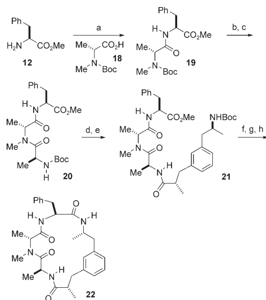
Scheme 3. Preparation of the geodiamolide analogue 22 . a) DCC, HOBT, amino acid 18 , THF, 0 \rightarrow 23 ^{\circ}\text{C} , 12 h (70%); b) TFA, \text{CH}_2\text{Cl}_2 , 23 ^{\circ}\text{C} ; c) PyBroP, i\text{Pr}_2\text{NEt} , N-Boc-L-Ala-OH ( 13 ), \text{CH}_2\text{Cl}_2 , 23 ^{\circ}\text{C} , 1 h (61%); d) TFA, \text{CH}_2\text{Cl}_2 , 23 ^{\circ}\text{C} ; e) EDCI, HOBT, amino acid 4 , \text{CH}_2\text{Cl}_2/\text{THF} , 0 \rightarrow 23 ^{\circ}\text{C} , 7 h (52%); f) NaOH, THF/ \text{H}_2\text{O} , 23 ^{\circ}\text{C} , 3 h (90%); g) TFA, \text{CH}_2\text{Cl}_2 , 23 ^{\circ}\text{C} , 1 h; h) TBTU, HOBT, i\text{Pr}_2\text{NEt} , DMF, 23 ^{\circ}\text{C} , 14 h (65%).
