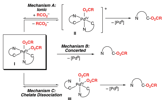
Scheme 6. Possible Mechanisms for C–O Bond-Forming Reductive Elimination from I
