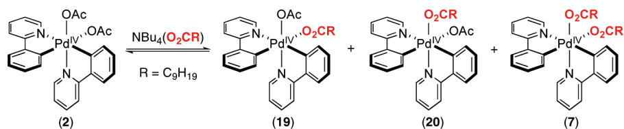
Scheme 9. Independent Synthesis of Complex 19 and ORTEP Picture of 19
