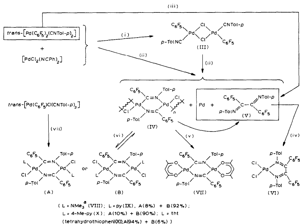
SCHEME 1. (i) Acetone, room temperature, 20 min; (ii) and (iii) Benzene reflux; (iv) PdCl_2(NCPh)_2 , benzene; (v) Tlaccac, CH_2Cl_2 ; (vi) L, CH_2Cl_2 ; (vii) Benzene reflux. a Possibly B isomer, as discussed in the text.
