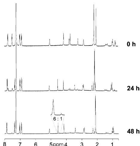
Figure 4. Monitoring of the 400.13 MHz ( \text{C}_6\text{D}_6 ) ^1\text{H} NMR spectrum of 4 in the 8.0–0.7 ppm region.
