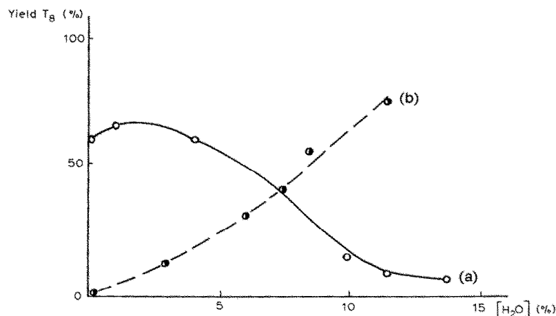
Fig. 3. Dependence of yield of T_8 on water concentration: (a) cyclorosiloxane:alkali ratio 1:1, (b) catalytic amount of alkali.
