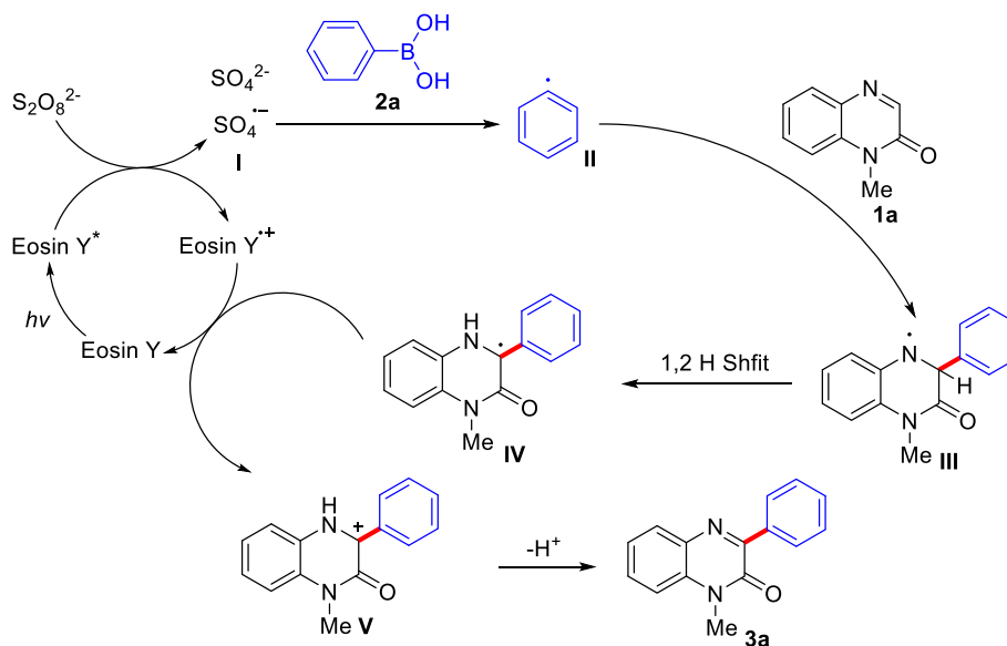
Scheme 3. Plausible mechanism.
