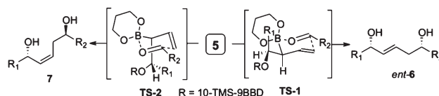
Scheme 2. Competitive Transition States Leading to ent -6 and 7
