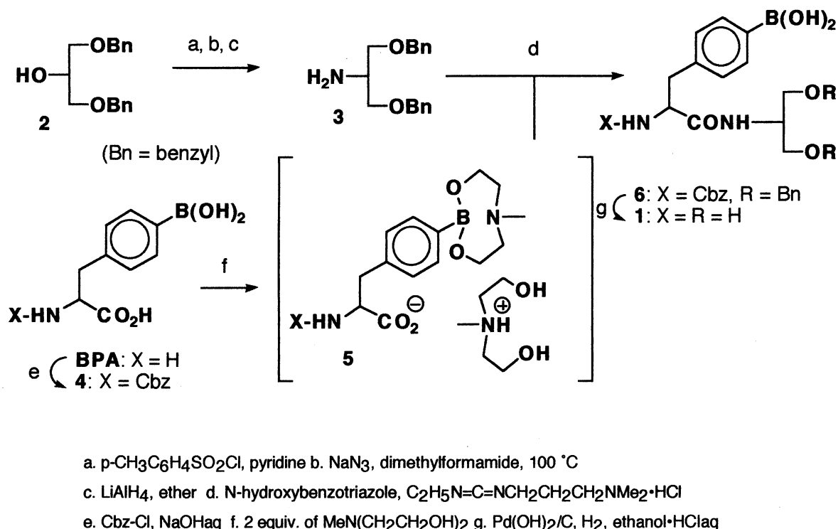
Scheme 1. Synthesis of 1.
