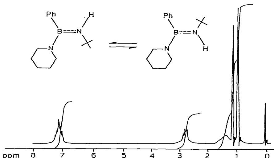
Fig. 2. ^1\text{H} NMR spectrum of \text{PhB}(\text{NH}-t\text{-Bu})\text{N-piperidine} .
