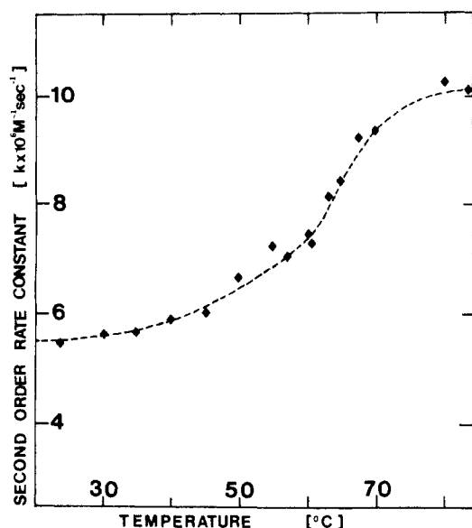
Figure 3. Temperature variation of the second-order rate constant obtained with pure (\text{C}_{18}\text{OCH}_2)_8\text{PcH}_2 ; \lambda_{\text{ex}} = 532 \text{ nm} .
