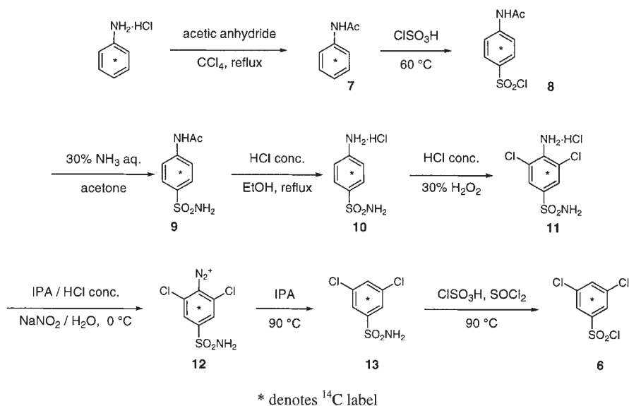
Scheme 2. Synthesis of sulfonyl chloride 6
