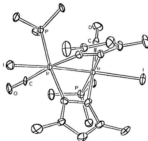
Fig. 1. Perspective view of [\text{Ir}(\text{CO})(\text{PhO})_3\text{P}]_2 . The I–Ir–Ir–I arrangement is approximately linear, the Ir–Ir bond length is 2.688 Å. (Phenyl rings omitted.)
