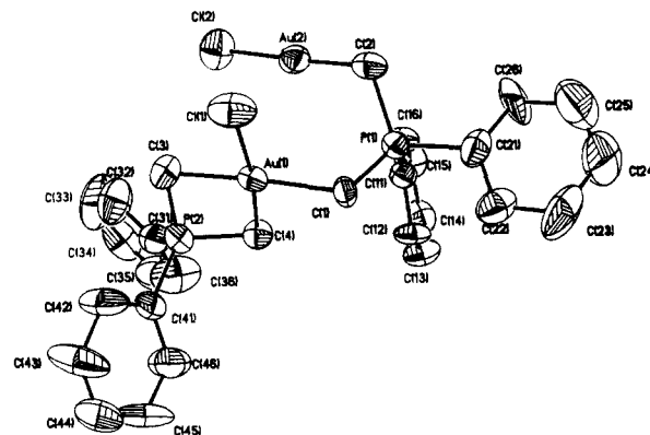
Figure 1. The molecular structure of the mixed-valence Au(III)/Au(I) dimer \text{ClAu}^{\text{I}}-\mu-[(\text{CH}_2)_2\text{PPh}_2]\text{Au}^{\text{III}}[\text{Cl}](\text{CH}_2)_2\text{PPh}_2 .
