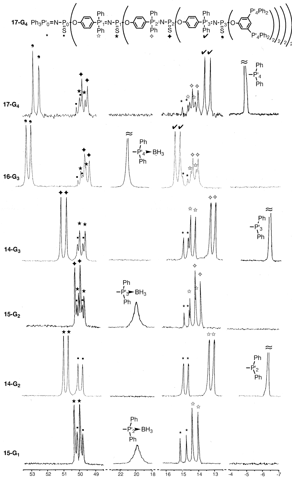
Fig. 1. 31 P-NMR spectra of all dendrimers from 15-G 1 to 17-G 4 .
