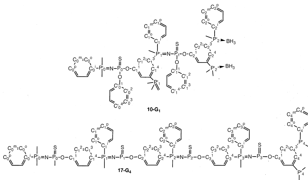
Fig. 3. Numbering used for NMR.
