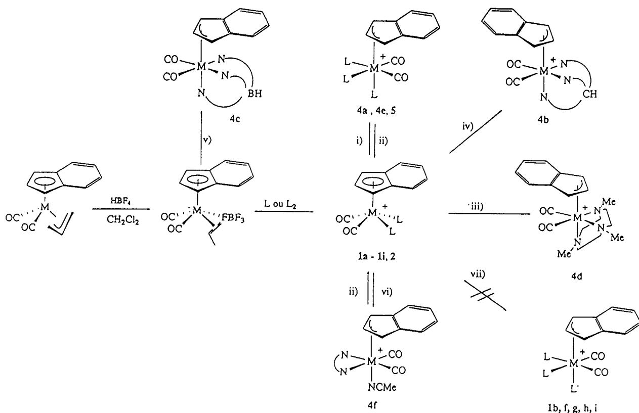
Scheme 1. (i) 1a , 2 in \text{NCMe} or 1d in dimethylformamide (DMF), at room temperature; (ii) 4a , 4e and 4f in \text{CH}_2\text{Cl}_2 ; (iii) \text{Me}_3\text{tacn} in \text{CH}_2\text{Cl}_2 ; (iv) 1c dissolved in \text{NCMe} at 45^\circ\text{C} ; (v) \text{KHB}(\text{pz})_3 in \text{CH}_2\text{Cl}_2 ; (vi) 1e in \text{NCMe} , \text{L}_2 = \text{en} ; (vii) 1b , 1f , 1g , 1h and 1i with an excess of \text{L} or \text{NCMe} at reflux.
