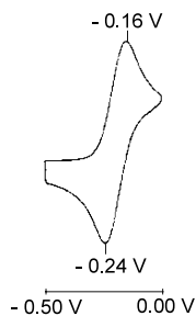
Fig. 3. Cyclic voltammogram of 4 in \text{CH}_2\text{Cl}_2 . Potentials are given in volts versus the saturated calomel electrode (SCE).
