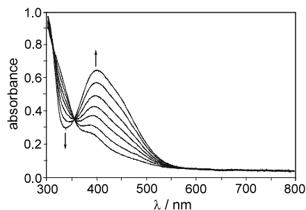
Fig. 5. UV-vis spectroscopic changes during gradual oxidation of 4 in an OTTLE cell.
