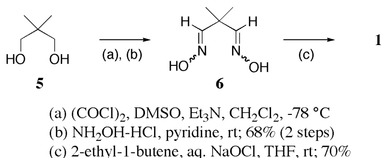
Scheme 2. Synthesis of 2,2-bis(isoxazolinyl)propane ( 1 )
